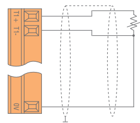
Thermocouple In
